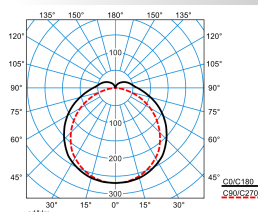
Deveo G3 6 DL 10-30/3ML-840 ET PC +LV (stage 1)
