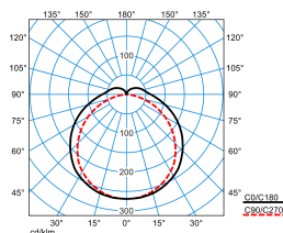
Deveo G3 6 DL 10-30/3ML-840 ET PC +LV (stage 3)
