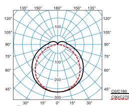
Deveo G3 6 DL 10-30/3ML-840 ET PC +LV (stage 2)
