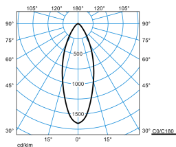
Amatris RC2 SRRFL 12-9MC ETBLE 05 + PC IP54 (stage 3)
