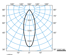
Amatris RC2 SRRFL 12-9MC ETBLE 05 (stage 2)
