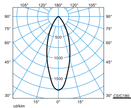
Amatris RC2 SRRFL 12-9MC ETBLE 05 (stage 3)
