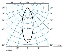
Amatris RC2 SRRFL 12-9MC ETBLE 05 + PC IP54 (stage 1)
