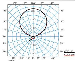
Luceos S-U PAW-IL 300-830 ETDI 05+LLWP (LEO2)
