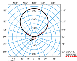
Luceos S-U PAW-IL 300-830 ETDI 05+LLWP (LEO1)
