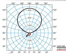
Luceos S-U PAW-IL 300-830 ETDI 05+LLWP (LEO2)
