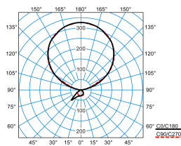
Luceos S-U PAW-IL 300-830 ETDI 05+LLWP (LEO1)
