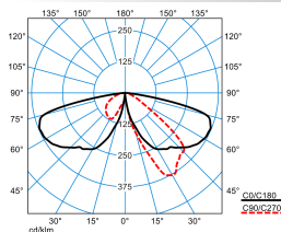
CS 19 C 100-AB2L/4200-730 4G1S ETDD (CLO initial value)
