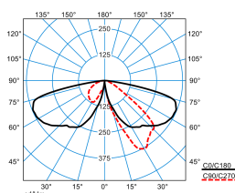
CS 19 C 100-AB2L/4200-730 4G1S ETDD (CLO end value)
