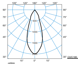
E-Line PRO 78 BV G2 RF-FL 40-EW M48 ETBLE 03 Blank
