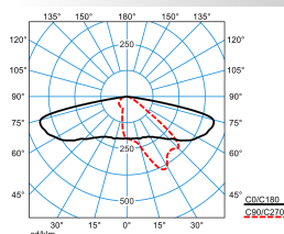
9301K AB2L-SLR1/2600-740 4G3 ET(CLO initial value)
