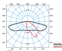
9301K AB2L-SLR1/2600-740 4G3 ET(CLO end value)
