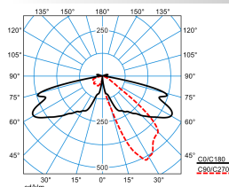
LTX P-AB2C-LRA/2600-730 4G1 ETDD (CLO initial value)
