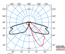
LTX P-AB2C-LRA/2600-730 4G1 ETDD (CLO end value)
