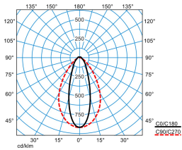
ELINE HE PN60-150 ML 830 L225 0 20
