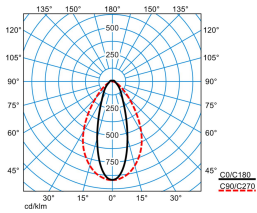
ELINE HE PN60-150 ML 830 L225 2 20
