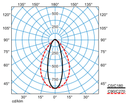
ELINE HE PN60-150 ML 830 L225 4 20
