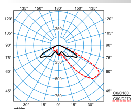
LnPlus 40-AM19L/15000-727 12G1 ETDD (CLO initial value)
