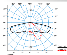
9301K AB2L-SLR3/3500-740 4G3 ET(CLO initial value)
