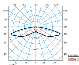
LIQ 50N-SB3L-SLR2/2200-730 2G1 ET (CLO end value)
