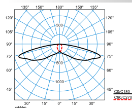
LIQ 50N-SB3L-SLR2/2200-730 2G1 ET (CLO initial value)
