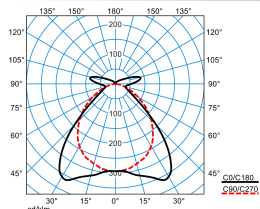
Tugra 12 PW 45-840 ETDD EB3 23
