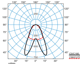
ELINE LDAN40-110 ML 840 L150 4 50
