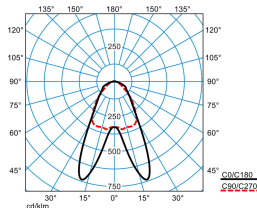
ELINE LDAN40-110 ML 840 L150 2 50
