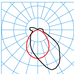
TugraHE Act 15 PAW 60-840 ETDD8 01 (ACTDCW) TX302961 ■ C0 - C180 ■ C90 - C270 DIN 5040: B40 UTE: 0.87 E + 0.13 T DLOR: 87 % ULOR: 13 % CEN Flux Code: 48 79 93 87 100 7 25 60 13
