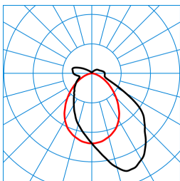
TugraHE Act 15 PAW 60-840 ETDD8 01 (ACTDSU) TX302747 ■ C0 - C180 ■ C90 - C270 DIN 5040: B40 UTE: 0.87 E + 0.13 T DLOR: 87 % ULOR: 13 % CEN Flux Code: 48 79 93 87 100 7 25 60 13
