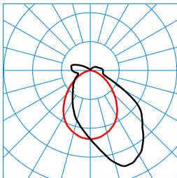
TugraHE Act 15 PAW 60-840 ETDD8 01 (ACTDWW) TX302914 ■ C0 - C180 ■ C90 - C270 DIN 5040: B40 UTE: 0.87 E + 0.13 T DLOR: 87 % ULOR: 13 % CEN Flux Code: 48 79 93 87 100 7 25 60 13
