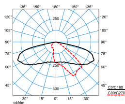
LIQ 50N-AB2L-LRA/1650-727 2G1 ETDD (CLO end value)
