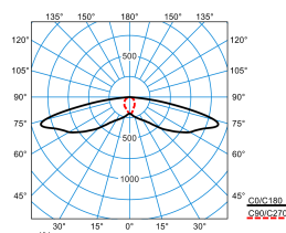
LIQ 50N-SB3L-SLR2/2200-727 2G1 ET (CLO end value)
