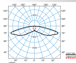
LIQ 50N-SB3L-SLR2/2200-727 2G1 ET (CLO initial value)
