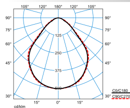
Parelia H-LM 11500-840 +LLWS 01 (LEO_direct_c90geo)
