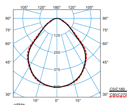
Parelia H-LM 11500-840 +LLWS 01 (LEO_direct_c270geo)
