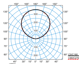
Parelia H-LM 11500-840 +LLWS 01 (LEO_indirect)
