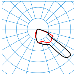
LIQ 70N-FR1L/6800-722 8G1 ET (CLO end value) TX778789 ■ C0 - C180 ■ C90 - C270 DIN 5040: A40 UTE: 1,00 F DLOR: 100 % ULOR: 0 % CEN Flux Code: 41 83 99 100 100
