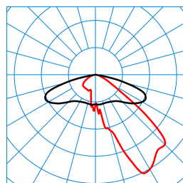
Publisca P2-AB2L/3200-740 4G1S ETDD (CLO initial value) TX300897 ■ C0 - C180 ■ C90 - C270 DIN 5040: A30 UTE: 1,00 G DLOR: 100 % ULOR: 0 % CEN Flux Code: 35 73 97 100 100
