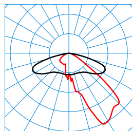
Publisca P2-AB2L/3200-740 4G1S ETDD (CLO end value) TX300437 ■ C0 - C180 ■ C90 - C270 DIN 5040: A30 UTE: 1,00 G DLOR: 100 % ULOR: 0 % CEN Flux Code: 35 73 97 100 100
