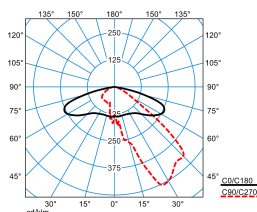
Publisca P2-AB2L/3200-740 4G1S ETDD (CLO initial value) TX300897 DIN 5040: A30 UTE: 1,00 G DLOR: 100 % ULOR: 0 % CEN Flux Code: 35 73 97 100 100
