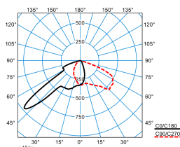
LIQ 50N-FL1L/4200-730 4G1 ET (CLO initial value) TX780461
