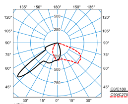
LIQ 50N-FL1L/4200-730 4G1 ET (CLO end value)
