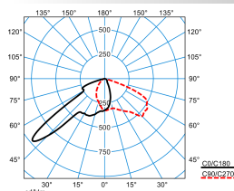
LIQ 50N-FL1L/4200-730 4G1 ET (CLO initial value)
