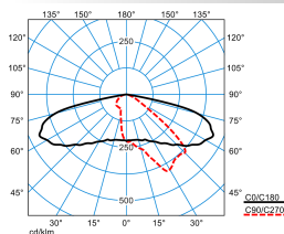
LIQ 50N-AB2L-LRA/2200-727 2G1 ETDD (CLO initial value)
