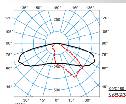
LIQ 50N-AB2L-LRA/2200-727 2G1 ETDD (CLO initial value)
