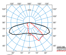
LIQ 50N-AB2L-LRA/2200-727 2G1 ETDD (CLO end value)
