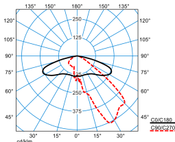
Publisca P2-AB2L-LR/3200-730 4G1S ET (CLO end value) TX301210 DIN 5040: A30 UTE: 1,00 G DLOR: 100 % ULOR: 0 % CEN Flux Code: 35 73 97 100 100
