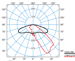
Publisca P2-AB2L-LR/3200-730 4G1S ET (CLO initial value) TX300732 DIN 5040: A30 UTE: 1,00 G DLOR: 100 % ULOR: 0 % CEN Flux Code: 35 73 97 100 100
