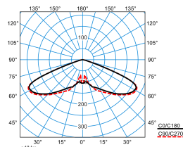
Publisca P1-RB6L/4200-740 6G1S ETDD (CLO end value)
