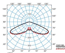
Publisca P1-RB6L/4200-740 6G1S ETDD (CLO initial value)
