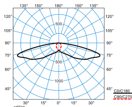
LIQ 50N-SB3L-LR-SLR2/2200-740 2G1 ET (CLO end value)
