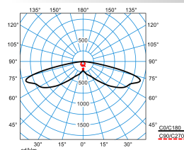
Publisca P2-SB3L/1200-730 2G1S ETDD (CLO initial value)
