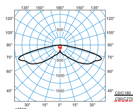
Publisca P2-SB3L/1200-730 2G1S
