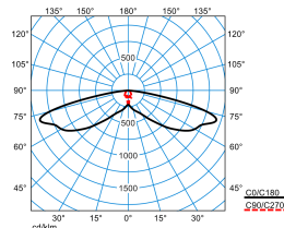
Publisca P2-SB3L/1200-730 2G1S ETDD (CLO end value)
