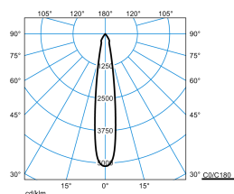
E-Line PRO 78 BV G2 RF-SP 30-BC M49 ETBLE 05 05
