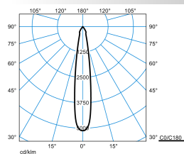
E-Line PRO 78 BV G2 RE-SP 30-BC M49 ETBLE 05 Blank
