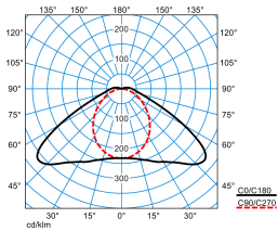
Nextrema G3 XB 40-840 ETDD+HFSX LV TWP
