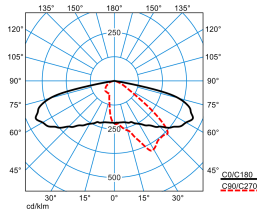
LIQ 50N-AB2L-LR/3200-730 4G1 ET (CLO initial value)
