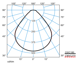
Siella G8 M84 PW19 28-44/4ML-840 ETDD (stage 3) TX562633
