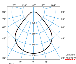
Siella G8 M84 PW19 28-44/4ML-840 ETDD (stage 4)
