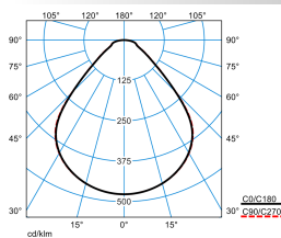
Siella G8 M84 PW19 28-44/4ML-840 ETDD (stage 1)
