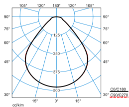
Siella G8 M84 PW19 28-44/4ML-840 ETDD (stage 4) TX562659
