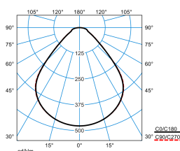
Siella G8 M84 PW19 28-44/4ML-840 ETDD (stage 3)
