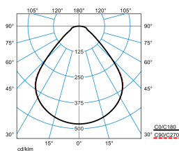
Siella G8 M84 PW19 28-44/4ML-840 ETDD (stage 2)
