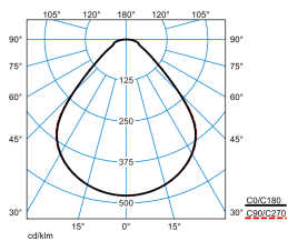
Siella G8 M84 PW19 28-44/4ML-840 ETDD (stage 2) TX562702
