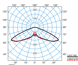
Publisca P1W-RB6L-LR/3800-740 6G1S
