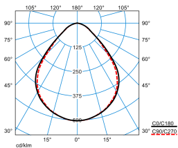
Opendo D1-L PW19 20-36/4/ML-830 ET 01 (2700lm) TX376571
