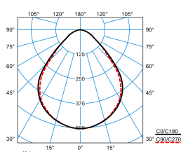
Opendo D1-L PW19 20-36/4/ML-830 ET 01 (3400lm)
