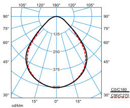
Opendo D1-L PW19 20-36/4/ML-830 ET 01 (2400lm) TX376570
