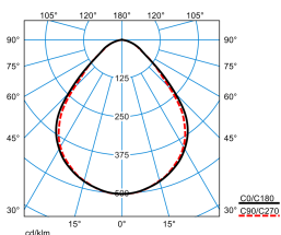
Opendo D1-L PW19 20-36/4/ML-830 ET 01 (3400lm) TX376572
