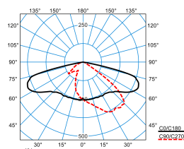
LIQ 70N-AB7L-SLR2/9100-740 10G1 ET(CLO end value)
