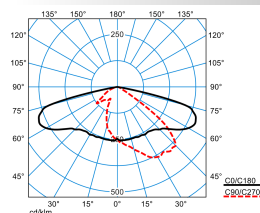
LIQ 70N-AB7L-SLR2/9100-740 10G1 ET(CLO initial value)
