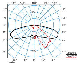
Publisca P2-AB2L-LR/2600-740 3G1S TX047752 DIN 5040: A30 UTE: 1,00 l DLOR: 100 % ULOR: 0 % CEN Flux Code: 34 71 96 100 100
