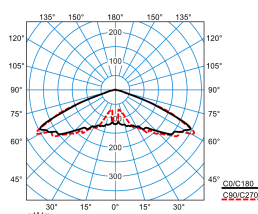
Publisca P1W-RB6L/1200-730 2G1S ETDD (CLO end value)
