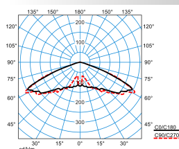
Publisca P1W-RB6L/1200-730 2G1S ETDD (CLO initial value)
