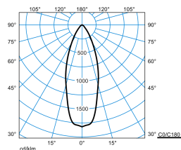
Amatris RC1 SRRFL 4/8/ML-9MC ETDD 05 (stage 4)
