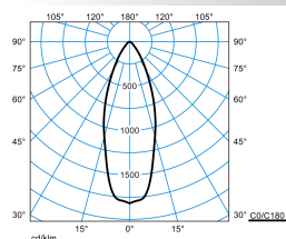
Amatris RC1 SRRFL 4/8/ML-9MC ETDD 05 (stage 1)
