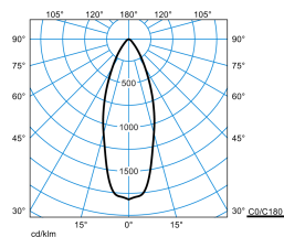
Amatris RC1 SRRFL 4/8/ML-9MC ETDD 05 (stage 2)
