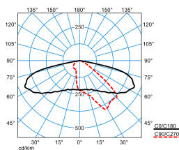
LIQ 50N-AB2L-LRA/1500-727 2G1 ETDD (CLO end value)
