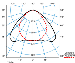
ELINE HE LVW60-160 ML 830 L225 2 20 DIN 5040 5 = A40 UGR I 5 = 25,3 UGR q 5 = 26,2 UTE 5 = 0.98 D + 0.02 T CEN Flux Code = 53 86 97 98 100 0 0 33 2
