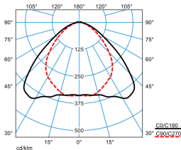
ELINE HE LVW60-160 ML 830 L225 4 20
