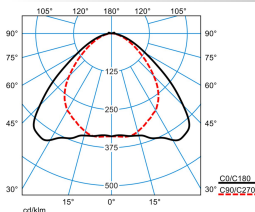
ELINE HE LVW60-160 ML 830 L225 0 20
