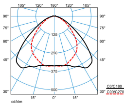
ELINE HE LVW60-160 ML 830 L225 2 20
