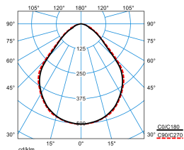
Parelia H-L 13000-830 01 (direct c90geo) TX057084
