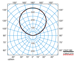
Parelia H-L 13000-830 01 (indirect) TX057085
