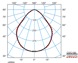
Parelia H-L 13000-830 01 (direct c270geo) TX057083
