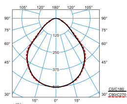
Parelia H-L 13000-830 +LM1 01 (direct c270geo) TX059576
