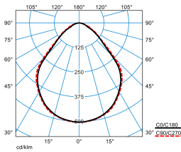
Parella H-L 13000-830 +LM1 01 (direct c90geo) TX059577
