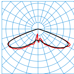
Publisca P2-RB6L-LRA/2600-740 3G1S ET (CLO end value) TX301223 ■ C0 - C180 ■ C90 - C270 DIN 5040: A20 UTE: 1,00 J DLOR: 100 % ULOR: 0 % CEN Flux Code: 20 57 98 100 100
