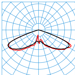
Publisca P2-RB6L-LRA/2600-740 3G1S ET (CLO initial value) TX301056 ■ C0 - C180 ■ C90 - C270 DIN 5040: A20 UTE: 1,00 J DLOR: 100 % ULOR: 0 % CEN Flux Code: 20 57 98 100 100
