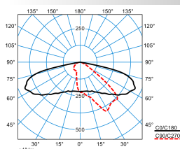
LIQ 50N-AB2L-LR/220/260/320-727 4G1 ET (CLO initial value)
