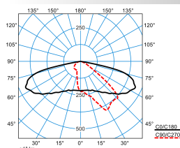
LIQ 50N-AB2L-LRA/22/26/32-730 4G1 ETDD (CLO end value) TX778485
