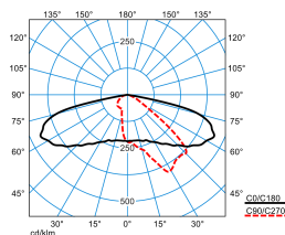
LIQ 50N-AB2L-LRA/22/26/32-730 4G1 ETDD (CLO initial value) TX778490
