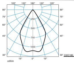
Inveria C 150 RB20R/2200-830 ETBLE +CAS TX776029
