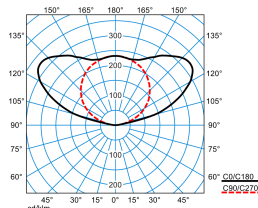
E-Line PRO 78HE I-UW 40-830ET L75 05 05
