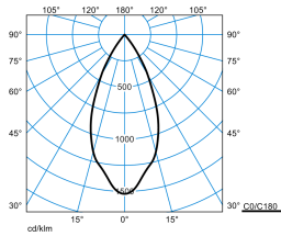
E-Line PRO 78 BV G2 RF-WFL 30-BC M49 ETBLE 01 01
