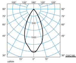
E-Line PRO 78 BV G2 RF-WFL 30-BC M49 ETBLE 01 Blank
