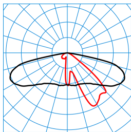
Publisca P2-AB2L/1800-730 2G1S ETDD (CLO initial value) TX301560 ■ C0 - C180 ■ C90 - C270 DIN 5040: A30 UTE: 1,00 G DLOR: 100 % ULOR: 0 % CEN Flux Code: 34 70 96 100 100
