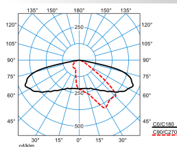
LIQ 50N-AB2L-LRA/3200-730 4G1 ETDD (CLO initial value)
