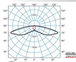
LIQ 50N-SB3L-LRA/1500-722 2G1 ETDD (CLO initial value)
