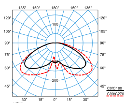
Publisca P1W-RBT-LRA/2200-740 3G1S ET (CLO initial value) TX300933 DIN 5040: A20 UTE: 0.99 l + 0.01 T DLOR: 99 % ULOR: 1 % CEN Flux Code: 26 63 91 99 100 0 0 0 1
