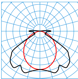
Nextrema G3 HE B 40-840 ETDD TWP TX768274
