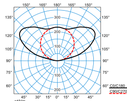
E-Line PRO 78HE I-UW 30-840ET L75 03 03
